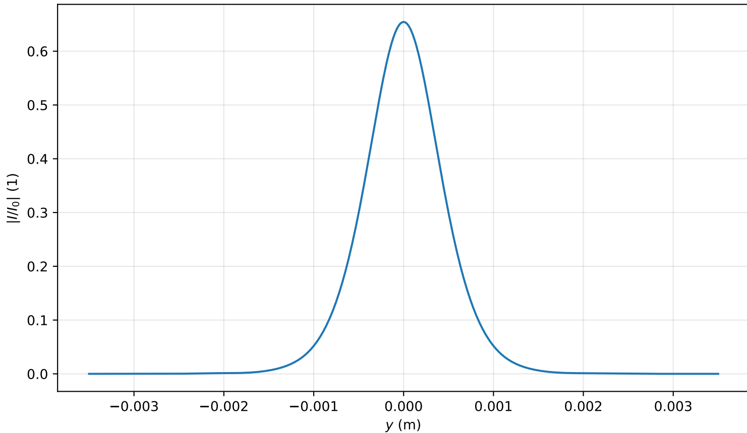
Intensity profile I(x=0, y, z=3.821)/I_0 , \text{Pin}=0.7\text{Pcr} , artificial time
